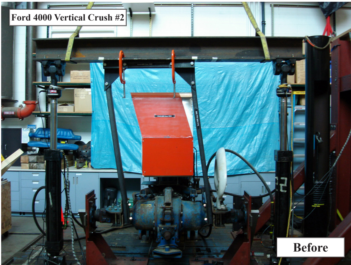
Ford 4000 Vertical Crush #2
